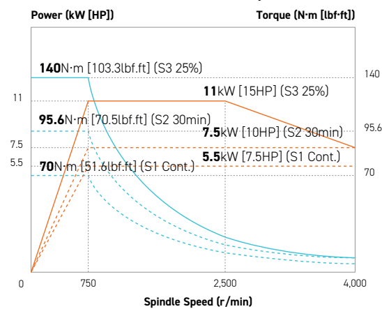
Mill Turret 4,000 rpm
